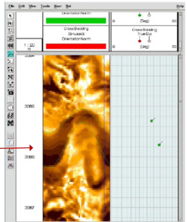
Figure 2. Imaging log confirming a large open fracture.
