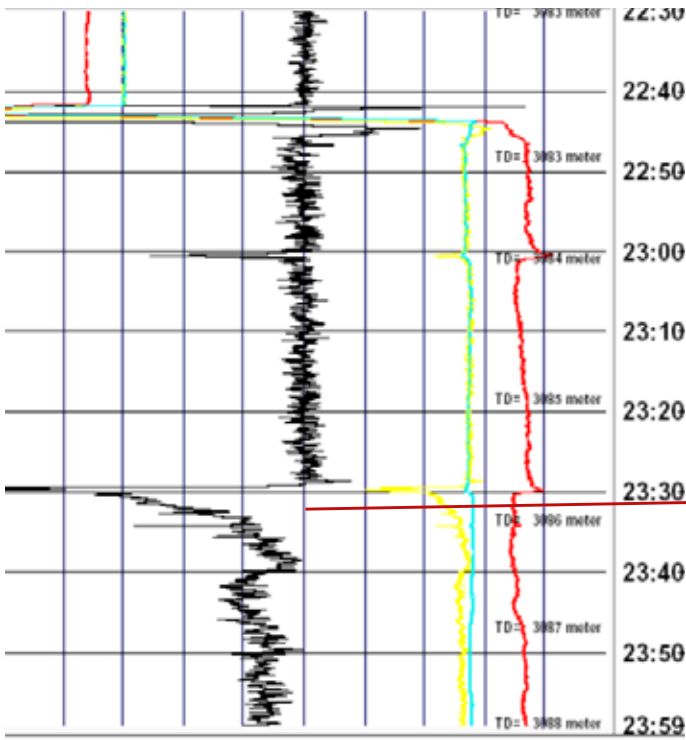
Figure 1. The curve in black is the Delta Flow which matches the signature of a natural open fracture in Figure 3.
